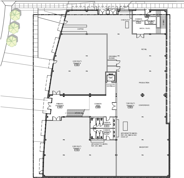
01 First Floor Plan
